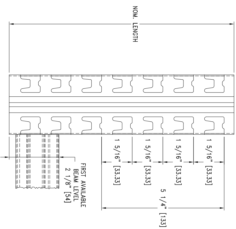
② STANDARD POSTS BEAM LEVELS CAN BE MOVED @ EVERY 1 5/16" LEVEL TO LEVEL
