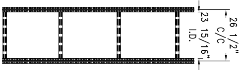
① FRAME WIDTHS
